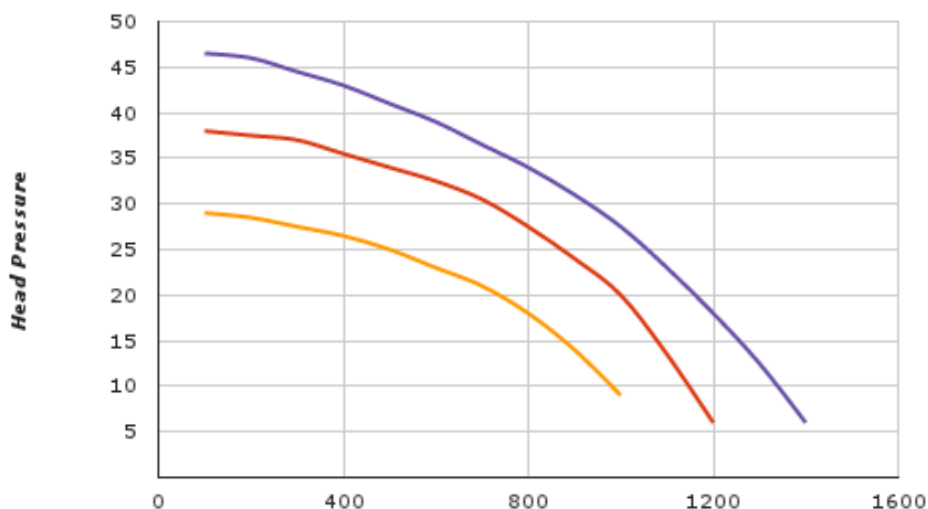
N-Tech Vertical Electric Pump - Series 20/50
